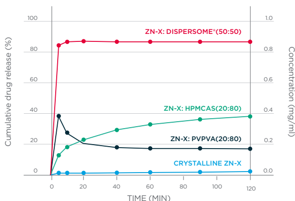
Drug dissolution of the poorly soluble drug, ZN-X, from different amorphous solid dispersions.
